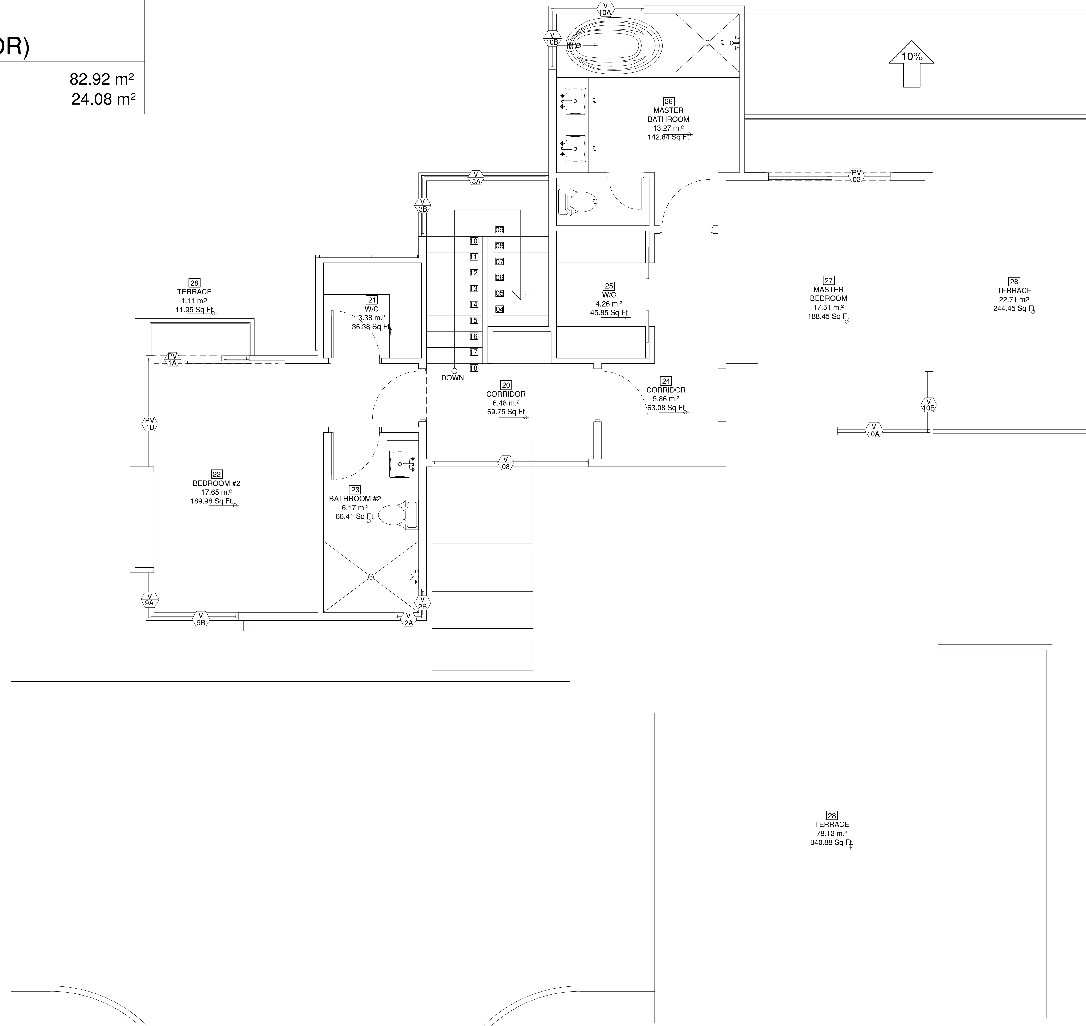
FLOOR PLAN FIRST FLOOR
