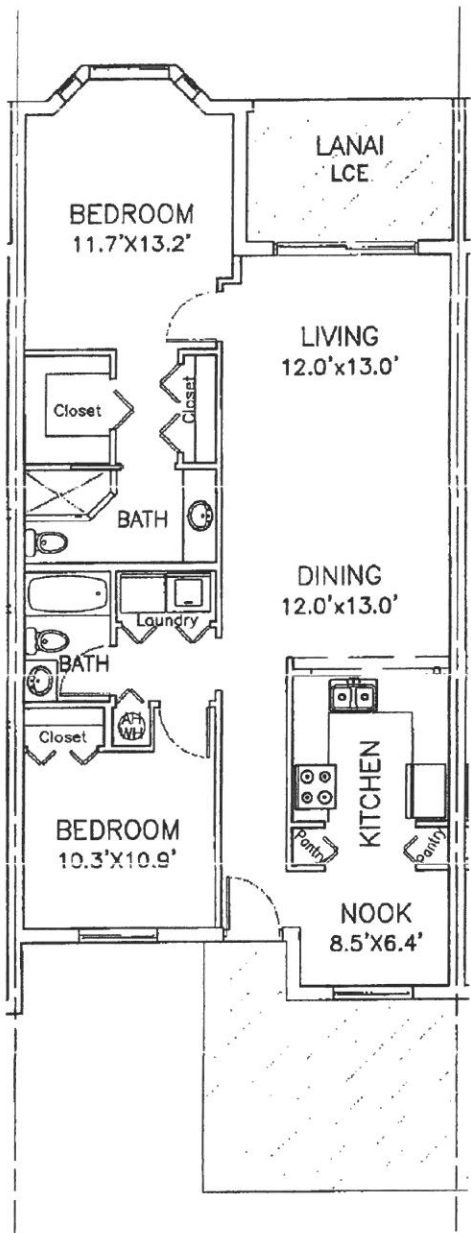
FLOOR PLAN
